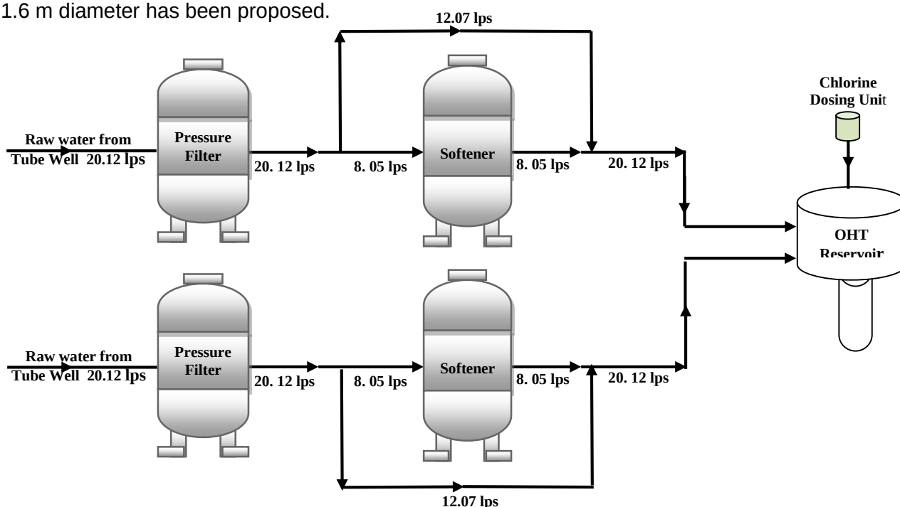
Figure IV-2: Schematic Diagram of Treatment Process
