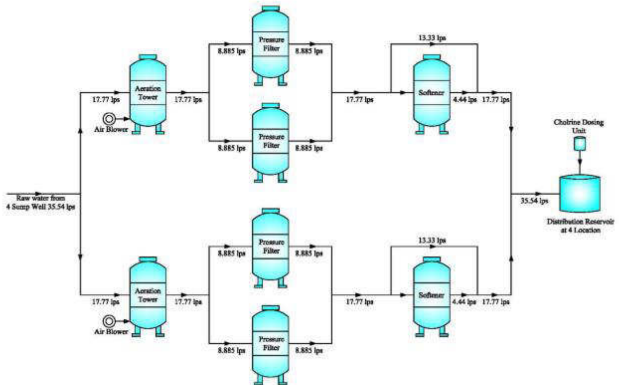
Figure IV-2-A: Schematic Diagram of Treatment Process for Mehelkuna System (System A)
