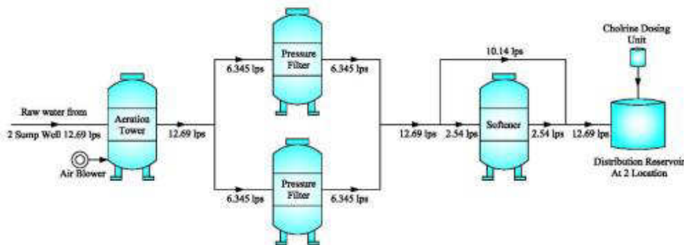
Figure IV-2-B: Schematic Diagram of Treatment Process for Botechaur System (System B)
